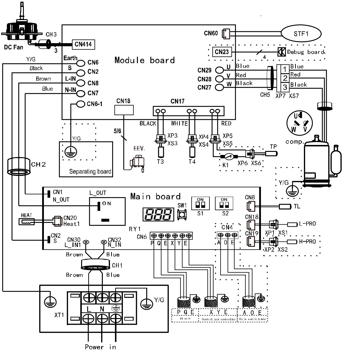
Figure 2-5.1: 28 model wiring diagram
