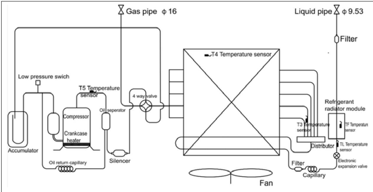
Figure 2-4.2: 36/42 model Piping diagram
