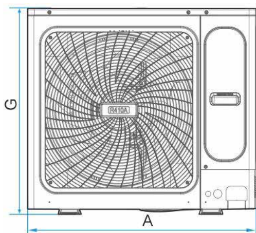
Figure 2-2.3: 28/36 model front view Dimensions
