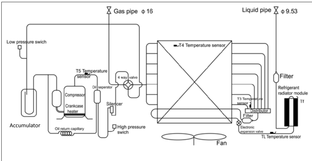
Figure 2-4.3: 48/56 model Piping diagram
