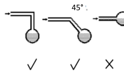
Figure 3-5.3: Branch drain piping joining main drain piping
