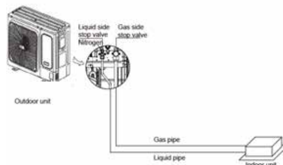
Figure 3-4.11: Gastightness test
