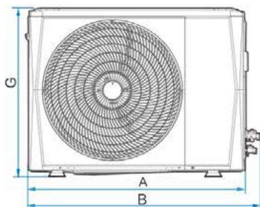
Figure 2-2.1: 28 model front view dimensions
