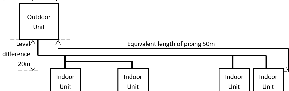
Figure 1-5.2: System diagram
