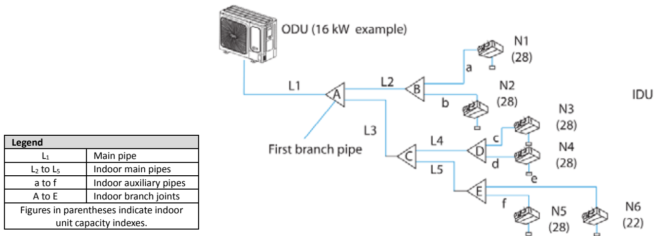
Figure 3-3.5: Refrigerant piping selection example
