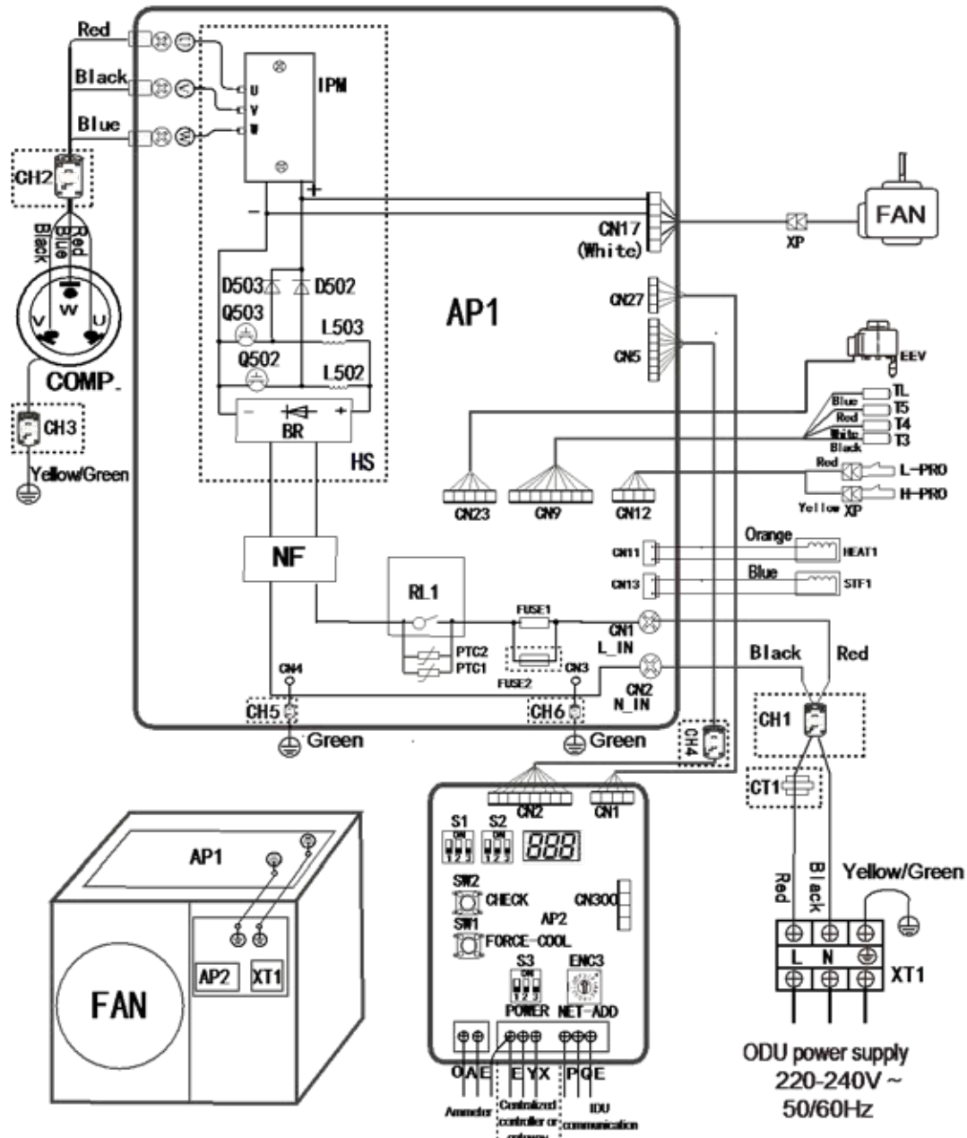
Figure 2-5.2: 36/42 model wiring diagram
