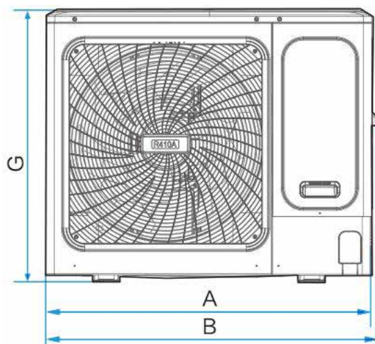
Figure 2-2.5: 48/56 model front view Dimensions
