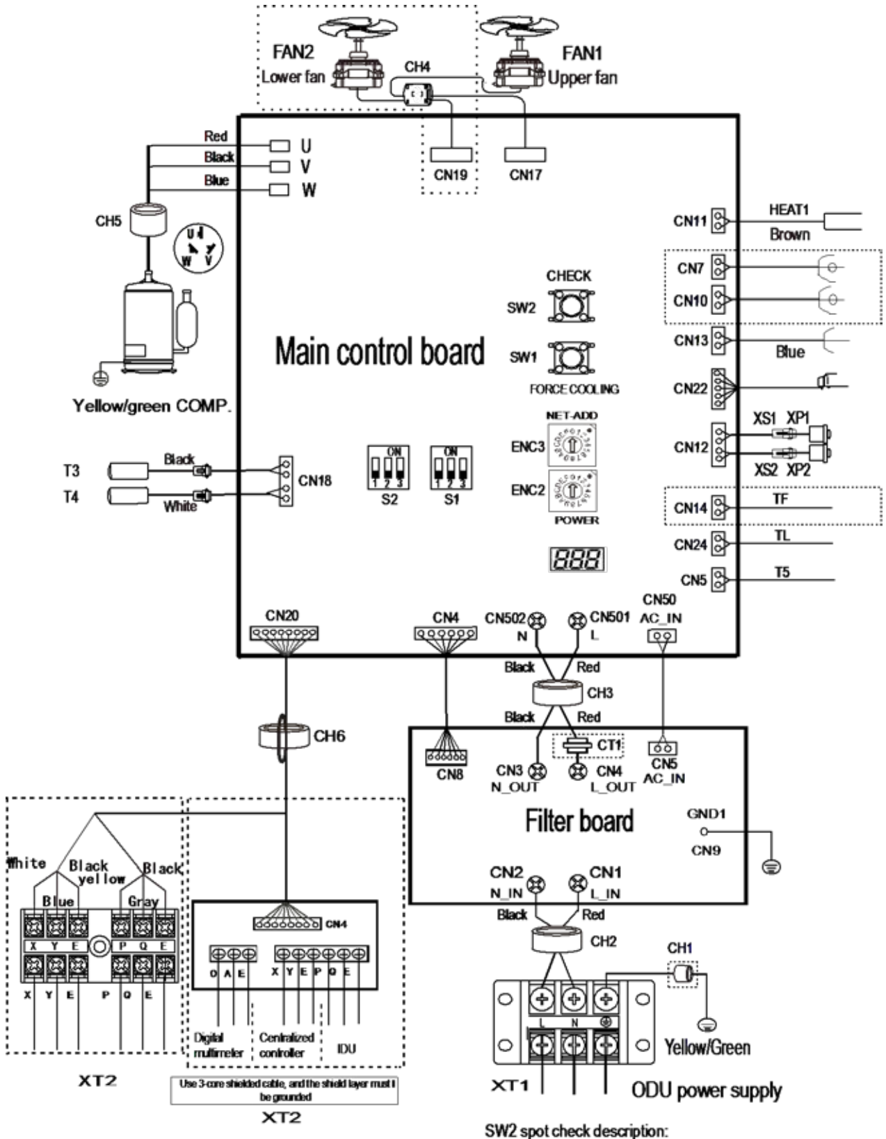
Figure 2-5.3: 48/56 model wiring diagram
